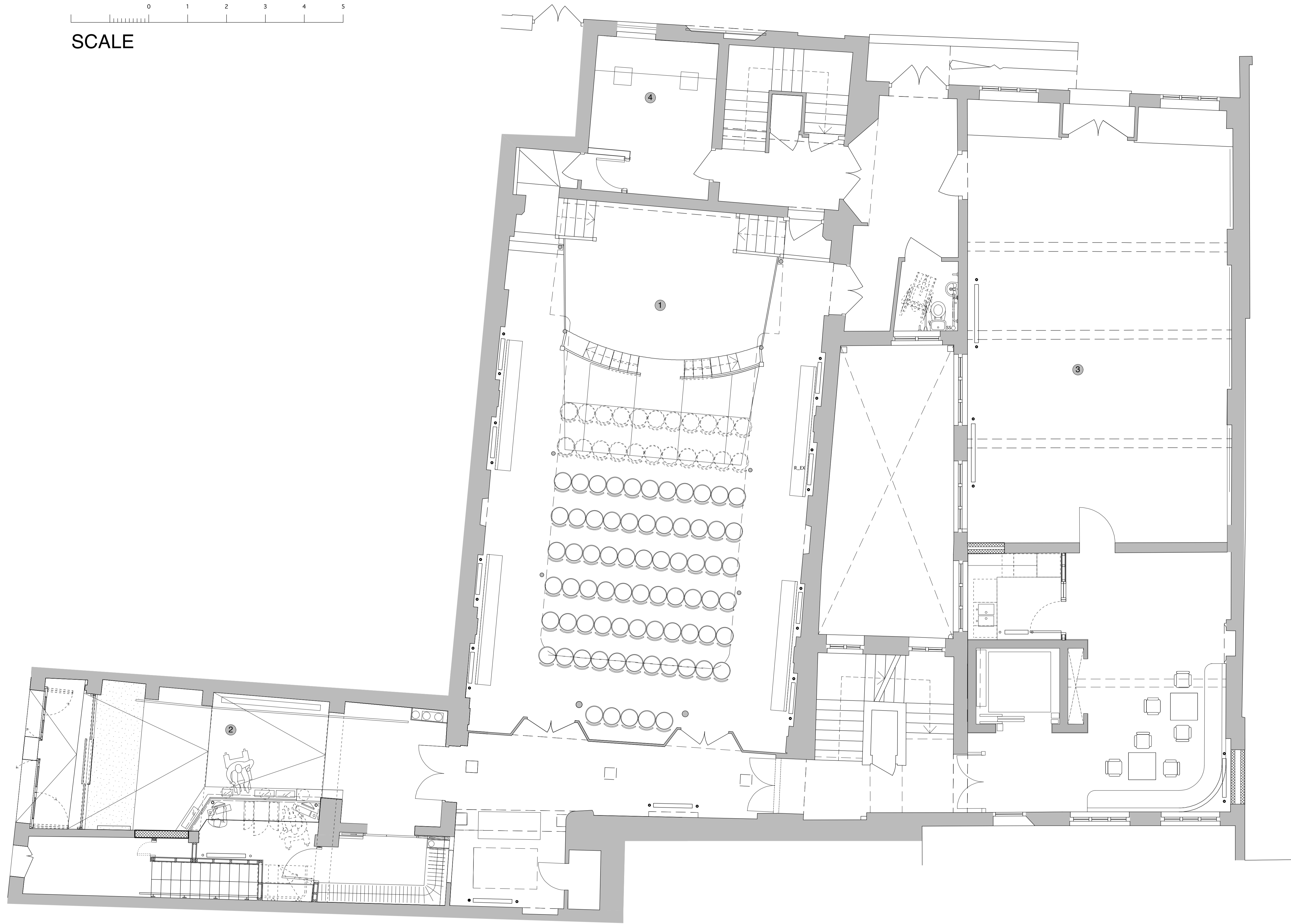
HOXTON HALL - GROUND FLOOR PLAN 1: 50 @A1
