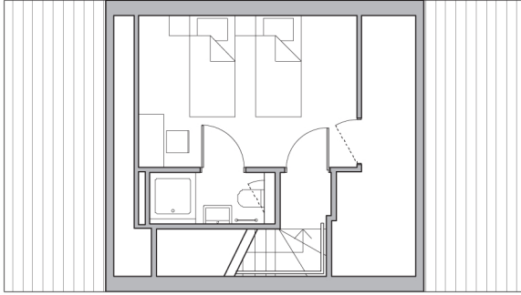
Four-bedroom house – first floor plan
